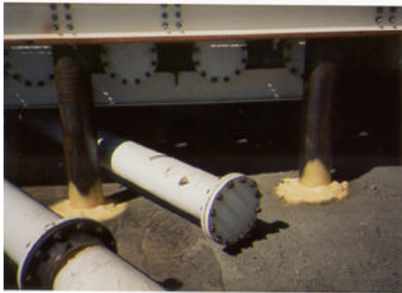
USING POLYSHIELD SS-100™ AND POLYURETHANE FOAM ON GEOTEXTILE FABRIC TO REPAIR AND EXTEND URETHANE LINER
